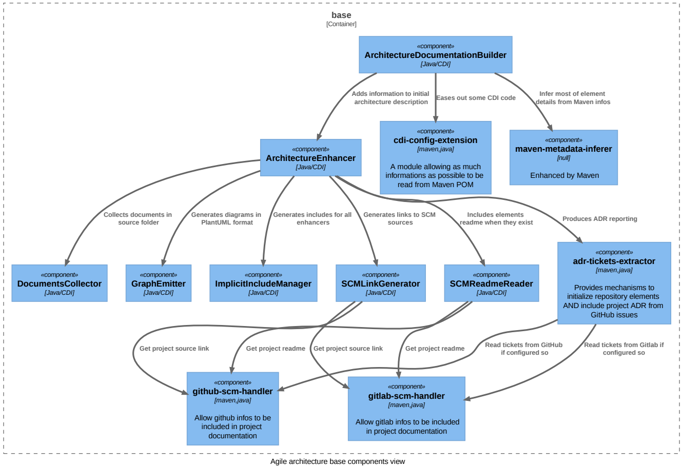
Agile architecture base components view
